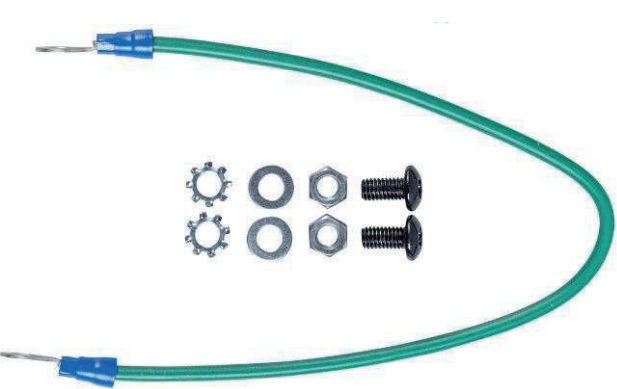
■ 700-017 CABINETGRKIT Grounding Kit
